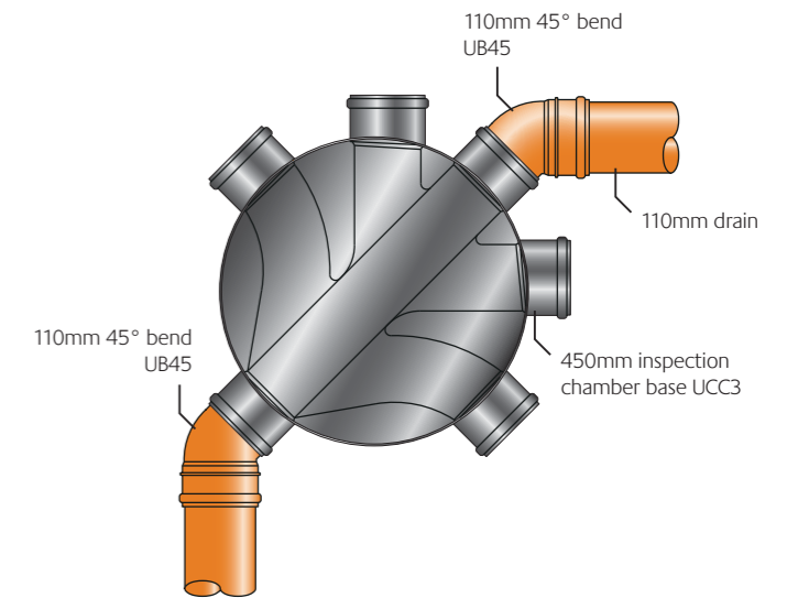
Typical 450mm inspection chamber 90° change of direction
