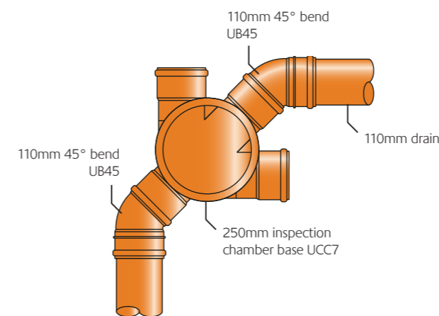
Typical 250mm inspection chamber 90° change of direction
